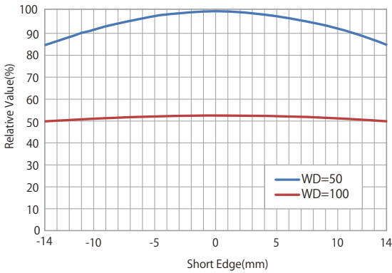
Lateral Direction(IDBA-RK600W)
