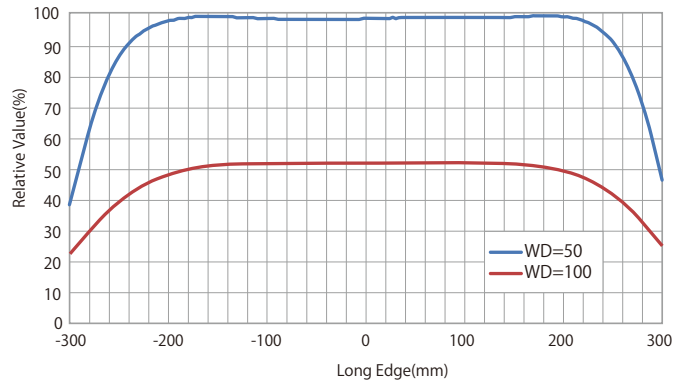
Longitudinal Direction(IDBC-RE300W)
