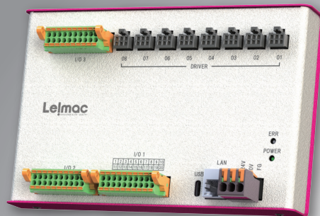
Trigger Pulse Controller Unit
